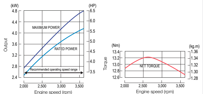
Power Curves
